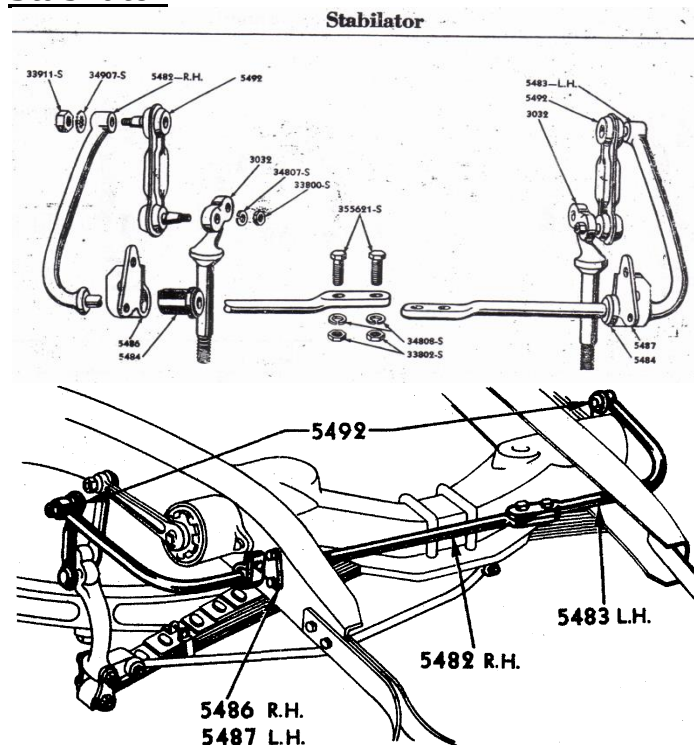
TORSION TYPE STABILIZER, 1940-1 LINCOLN-ZEPHYR, 1941 LINCOLN
