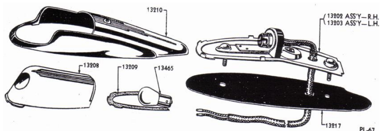
PARKING LAMP (1941)
