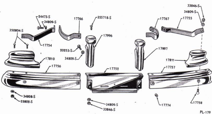
FRONT BUMPER (5EH-17748).
