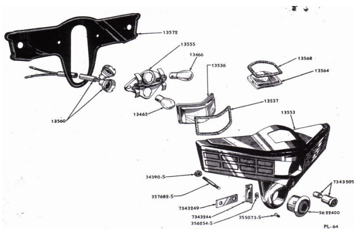
REAR LICENSE AND STOP LAMP (1946-48)
