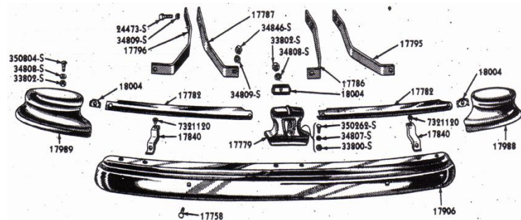
REAR BUMPER (5EH-17778-A)
