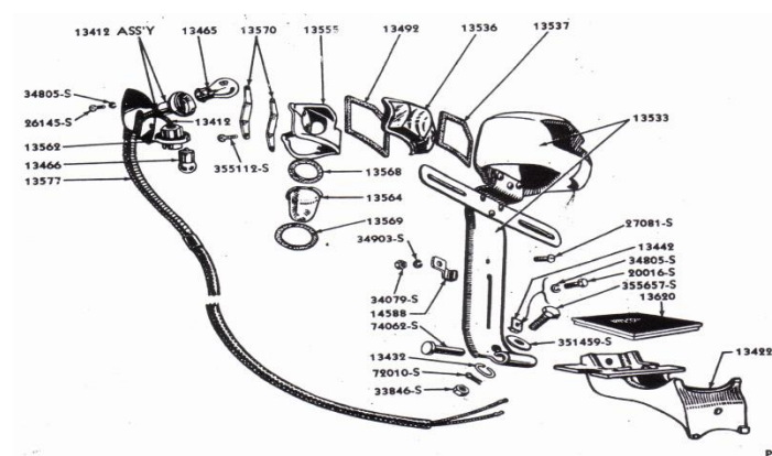
REAR LICENSE LAMP (1942-48 CONTINENTAL)
