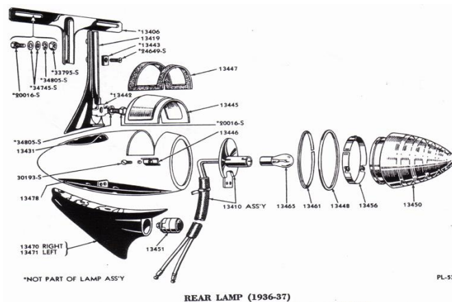
REAR LAMP (1936-37)
