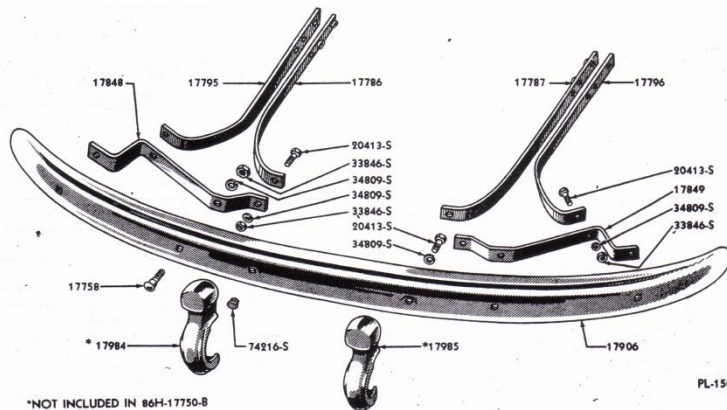
FRONT BUMPER KIT (86H-17750-B)
